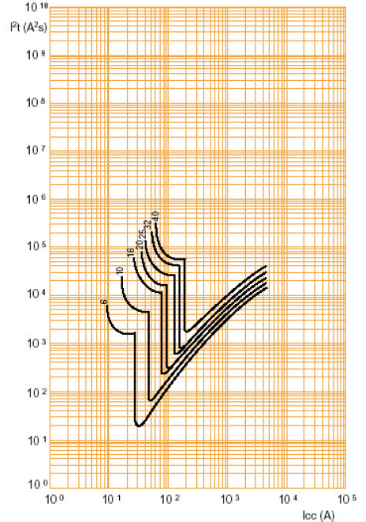
Btdin 45 1P+N 230V a.c. (1 module) - characteristic "B"
