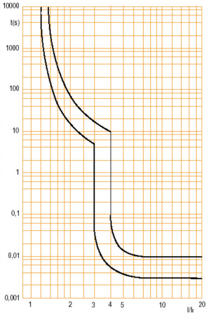
Btdin 45/60 - characteristic B
