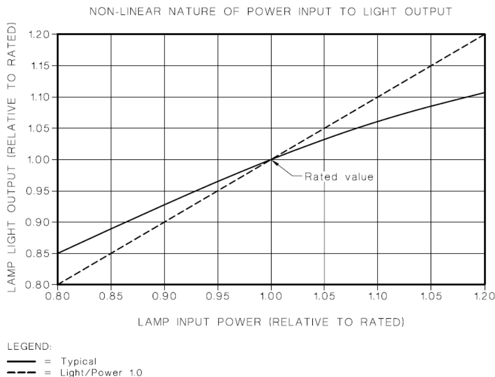
Figure F.2 — Variation of light output with lamp power
