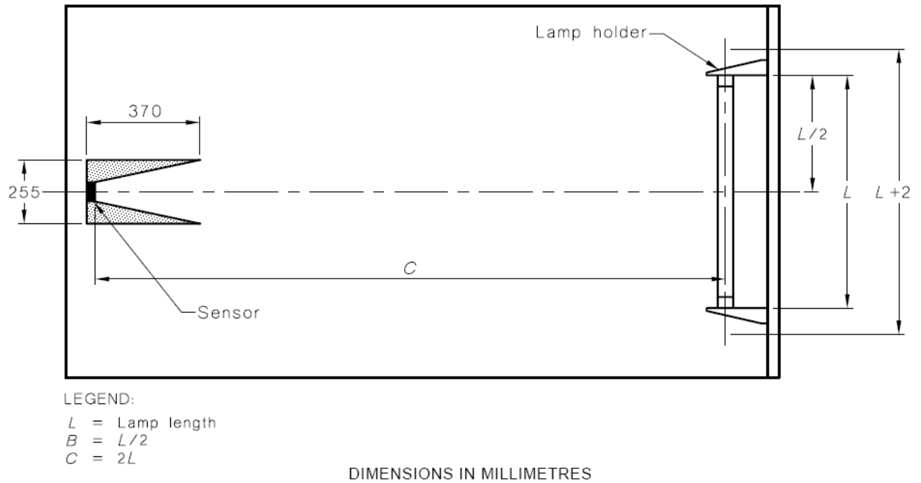
Figure D.2 — Top view of light output measurement system
