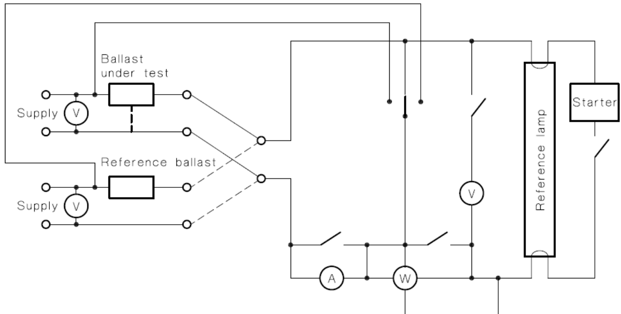
Figure E.1 Measurement of two-wire ballast-lamp circuits
