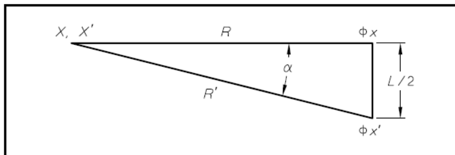
Figure D.3 — Configuration of lamp and photocell sensor
