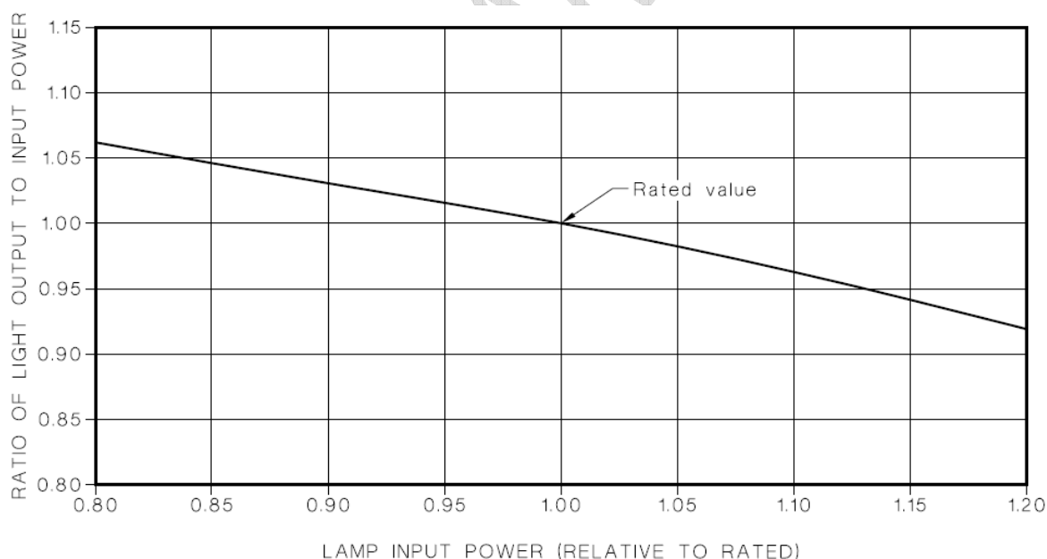
Figure F.1 — Variation of lamp efficiency with lamp input power
